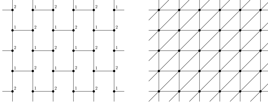
Figure 11: Representation of the hexagonal, (6^3) , lattice and its dual, the triangular lattice, (3^6)
