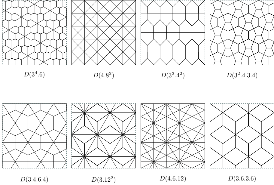
Figure 2: The Laves lattices
