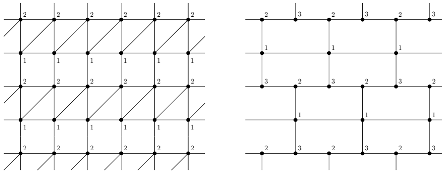
Figure 4: Representation of the (3^3.4^2) lattice and its dual
