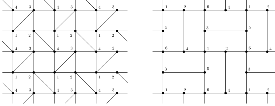
Figure 5: Representation of the (3^2.4.3.4) lattice and its dual
