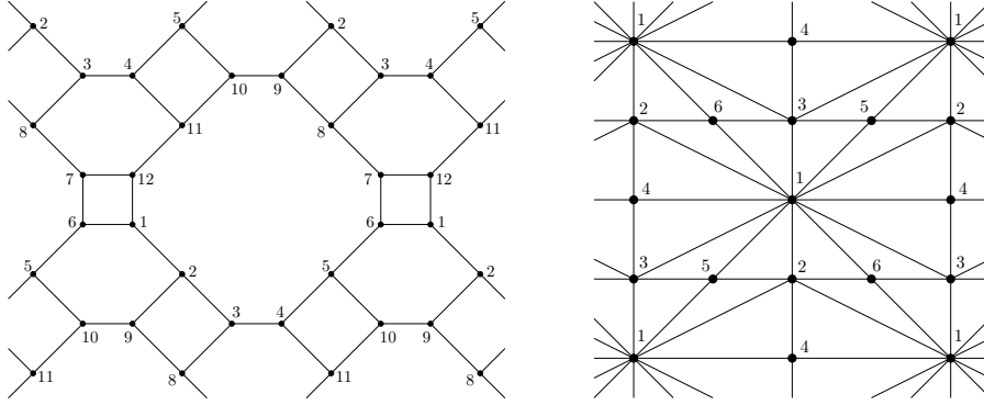
Figure 9: Representation of the (4.6.12) lattice and its dual
