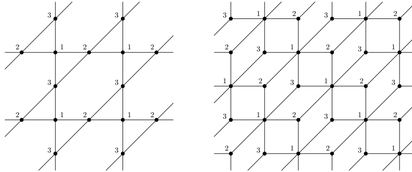
Figure 12: Representation of the (3.6.3.6) lattice and its dual
