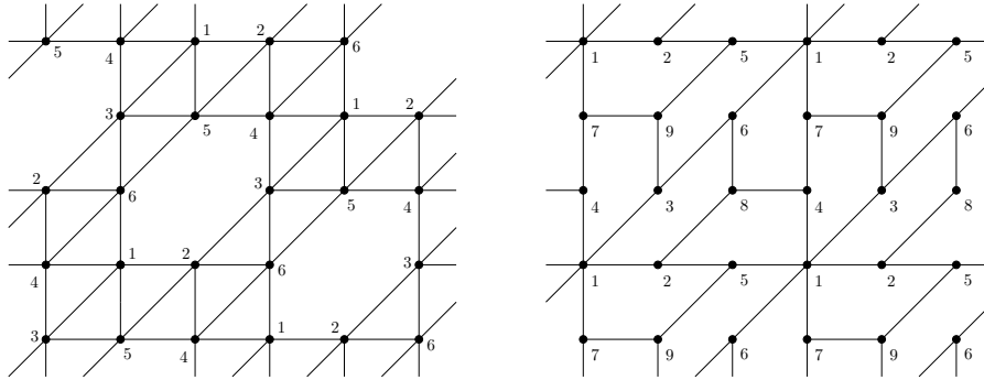
Figure 6: Representation of the (3^4.6) lattice and its dual
