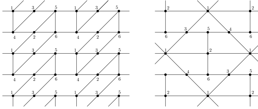
Figure 13: Representation of the (3.4.6.4) lattice and its dual
