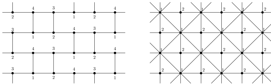
Figure 10: Representation of the (4.8^2) lattice and its dual
