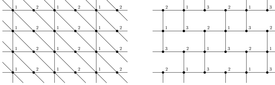
Figure 7: Representation of the Bow-tie lattice and its dual
