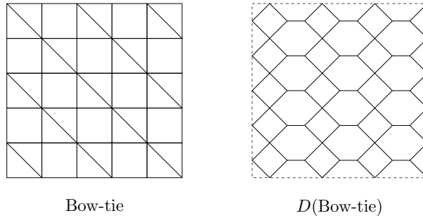
Figure 3: The Bow-tie lattice and its dual
