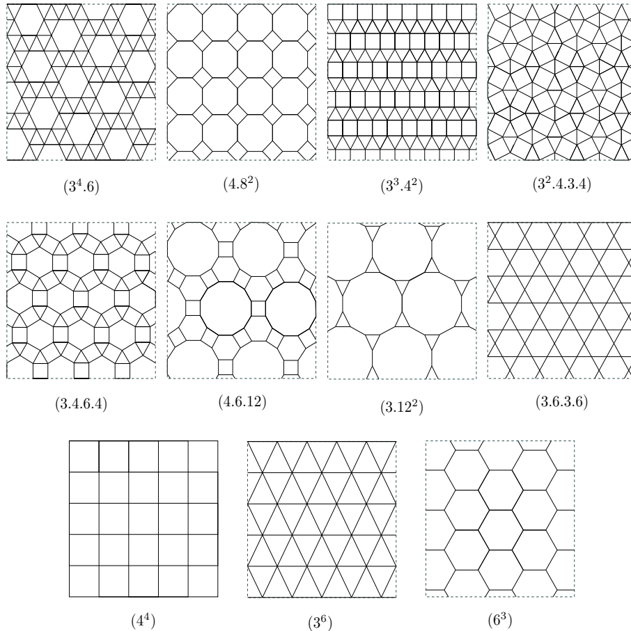
Figure 1: The Archimedean lattices
