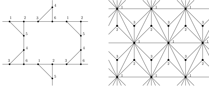
Figure 8: Representation of the (3.12^2) lattice and its dual
