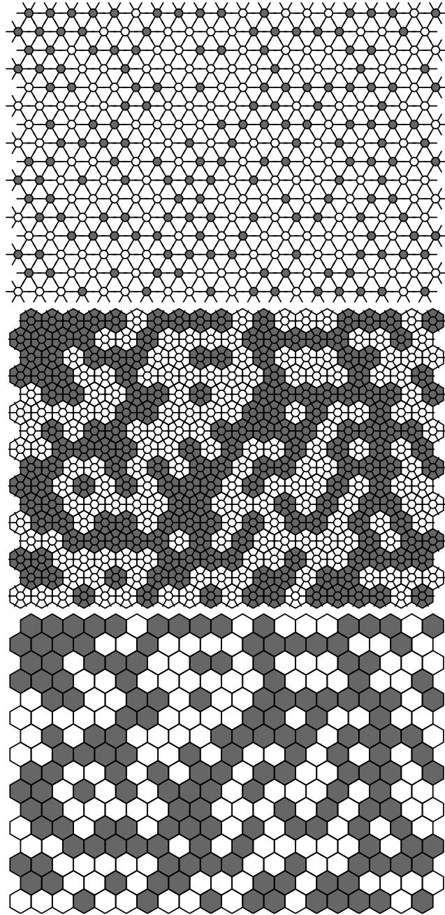
Figur 1: This figure explains how we get from a percolation configuration on the triangular lattice, to a percolation configuration on the faces of the hexagonal lattice. Black represents open vertices, while white represents closed.
