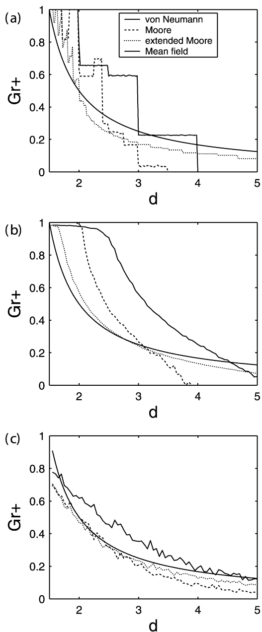
FIGURE 3 (a) Hawk–Dove interaction scenario obtained according to Table II with parameters b = 1 , c = 0.5 , and e = 1 . The equilibrium proportion of growth promoters ( Gr+ ) in the population is depicted as a function of increasing values of d . Competition for reproduction is fully deterministic and updating is semi-synchronous with individual mortality 0.1. The population was initiated with a proportion of growth promoters of 0.1. Thin solid line shows the mean field result according to Eq. (4). Thick solid, dashed, and dotted lines represent the von Neuman neighbourhood, the Moore neighbourhood, and the extended Moore neighbourhood, respectively. (b) As in Fig. 3a but probabilistic reproduction. (c) As in Fig. 3a but probabilistic reproduction and asynchronous updating.
