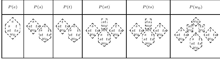
FIGURE 1. Indecomposable projectives in \mathcal{O}_0
