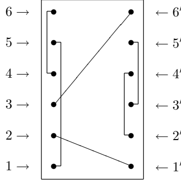
Figure 1: The element \{\{1, 5\}, \{4, 6\}, \{2', 4'\}, \{3', 5'\}, \{2, 1'\}, \{3, 6'\}\} of \mathfrak{B}_6 .
