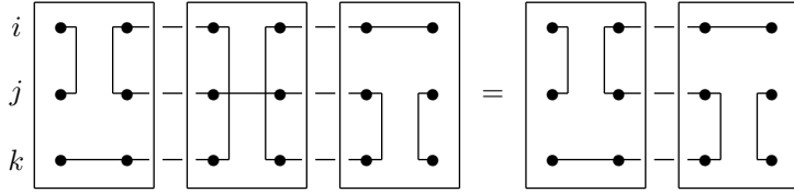
Figure 5: An example illustrating the relation (6).
