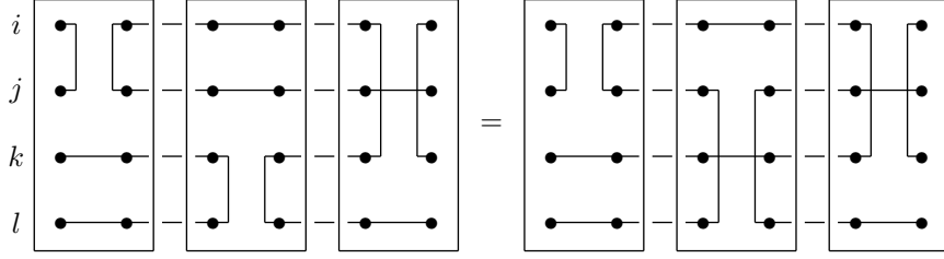
Figure 7: An example illustrating the relation (8).
