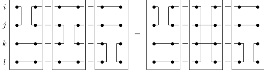
Figure 4: An example illustrating the relation (5).
