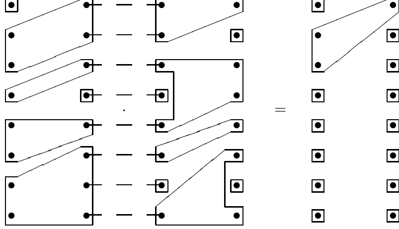
FIGURE 4. Elements of \widetilde{\mathcal{P}\mathcal{I}}_8^* and their multiplication.
