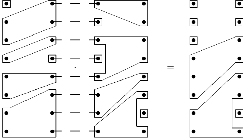
FIGURE 2. Elements of \mathcal{PI}_8^* and their multiplication.
