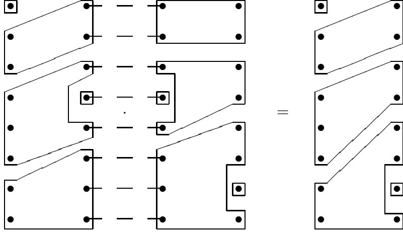
FIGURE 3. An example of a non-trivial product in \widehat{\mathcal{PI}}_8^* .
