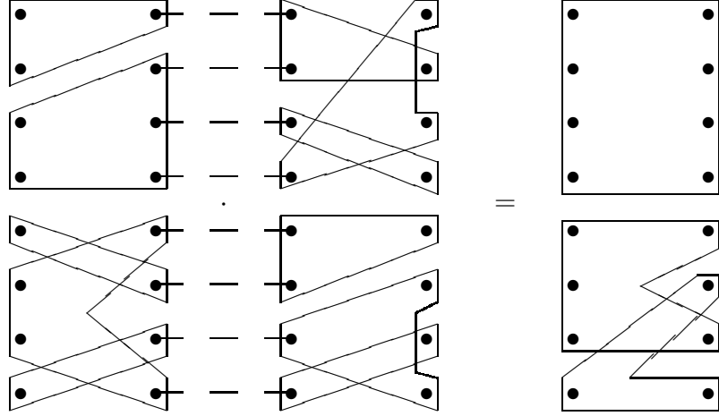
FIGURE 1. Elements of \mathcal{I}_8^* and their multiplication.
