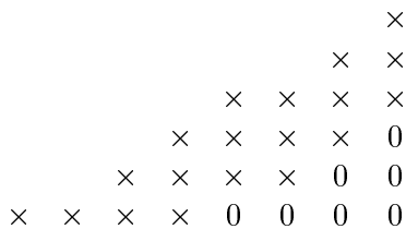
Figure 1: D^*(4, 2, 1) marked with 0; SQ(4, 2, 1; 4) marked with \times
