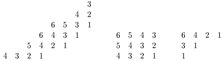
Figure 2: SQ(4, 2, 1; 4) , R(3, 4) and D(4, 2, 1) with hook lengths
