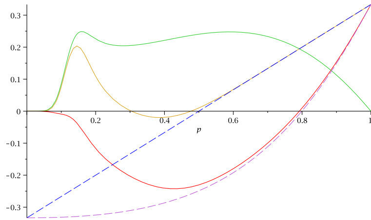
FIGURE 2. The solid curves are the covariance for \vec{G}(30, p) , middle curve, which by Fact 8.1 is the sum of the expected covariance for \vec{G}(30, M) , bottom, and \text{Var}(\mathbb{P}(A | M)) , top curve. The dashed curves are the asymptotic curves for \vec{G}(n, p) (straight line) and expected covariance for \vec{G}(n, M) . All curves normalized with 3(1 - p/2)^{2n-3} .
