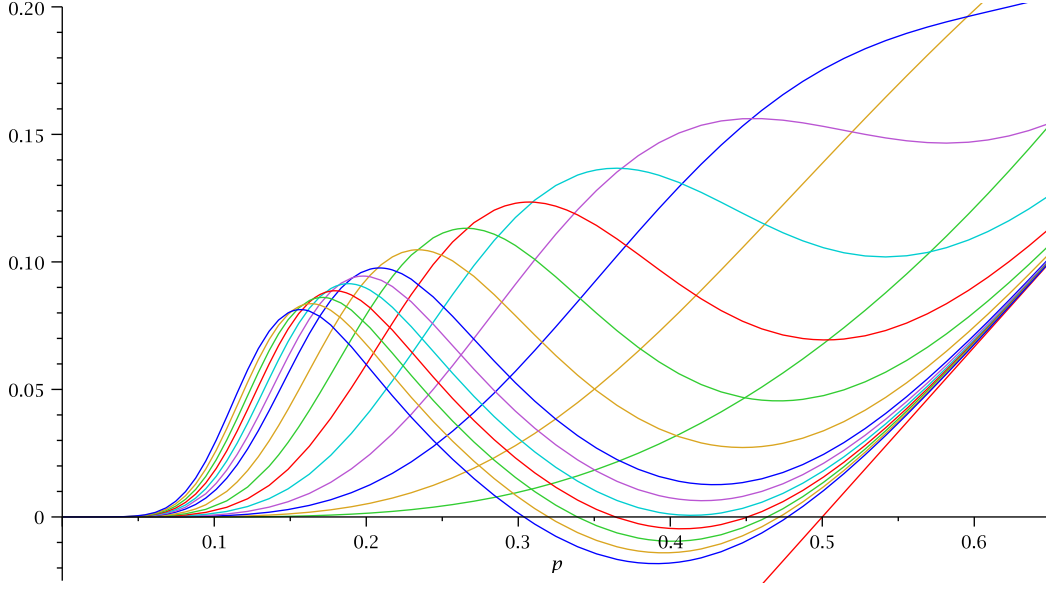
FIGURE 1. The relative correlation \frac{\mathbb{P}(a \nrightarrow s, s \nrightarrow b) - \mathbb{P}(a \nrightarrow s)\mathbb{P}(s \nrightarrow b)}{\mathbb{P}(a \nrightarrow s, s \nrightarrow b)} in \vec{G}(n, p) for n = 8, 10, 12, 14, 16, 18, 20, 22, 24, 25, 26, 27, 28, 29, 30 , and the asymptote (2p - 1)/3 . All curves are negative for very small p . For n \geq 27 we get three zeros.
