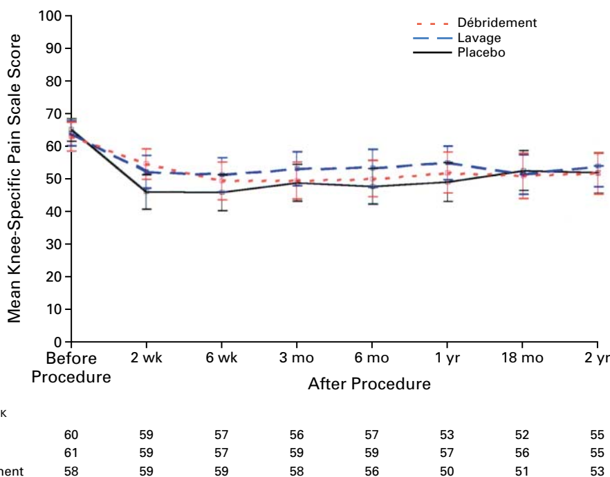
Figure 1. Mean Values (and 95 Percent Confidence Intervals) on the Knee-Specific Pain Scale. Assessments were made before the procedure and 2 weeks, 6 weeks, 3 months, 6 months, 12 months, 18 months, and 24 months after the procedure. Higher scores indicate more severe pain.
