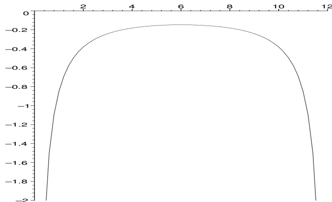
Figure 1: The function \pi^{-s}\Gamma(s)E(Y_{24}, s) for 0 < s < 12 .
