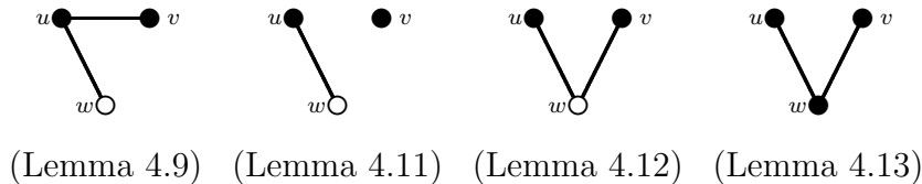
FIGURE 1. Subtemplates implying uniformity of G .
