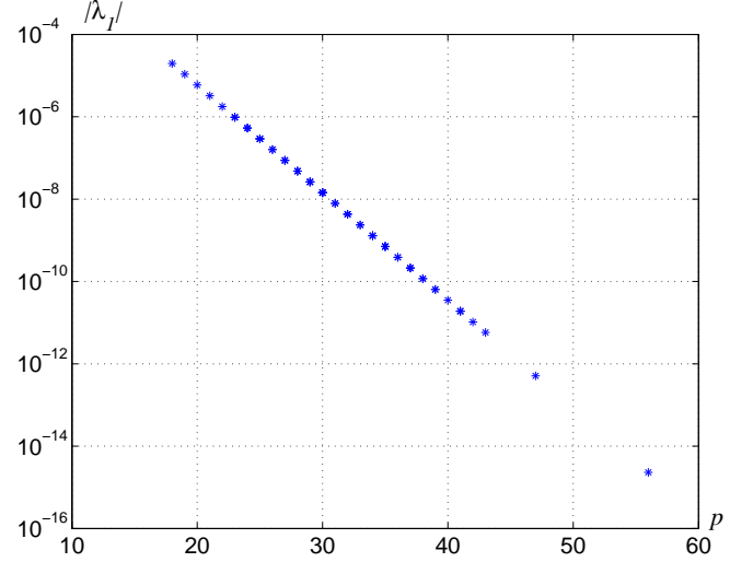
FIG. 7. The absolute value of the larger eigenvalue versus period p
