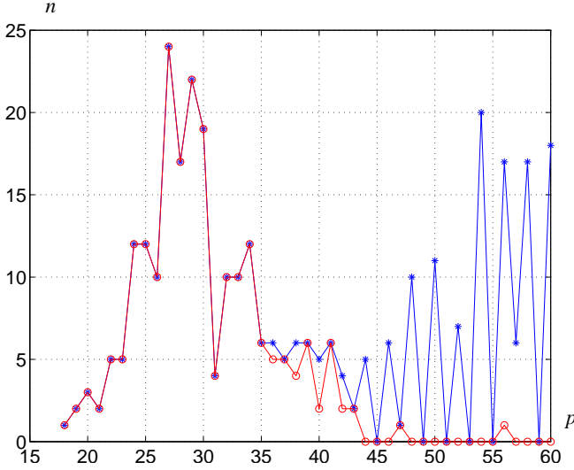
FIG. 5. The number of primary regions ( \circ ), and the total number of regions ( * ) found for each period p
