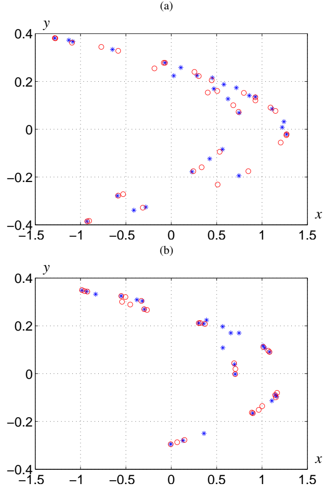
FIG. 12. (a) Period-28 sink for (a, b) = (1.39999995942006, 0.3) (*) and period-33 sink (a, b) = (1.3999991587739, 0.3) (○), (b) Period-26 sink for (a, b) = (1.4, 0.2999940739782) (*) and period-29 sink (a, b) = (1.4, 0.299993405894) (○)
