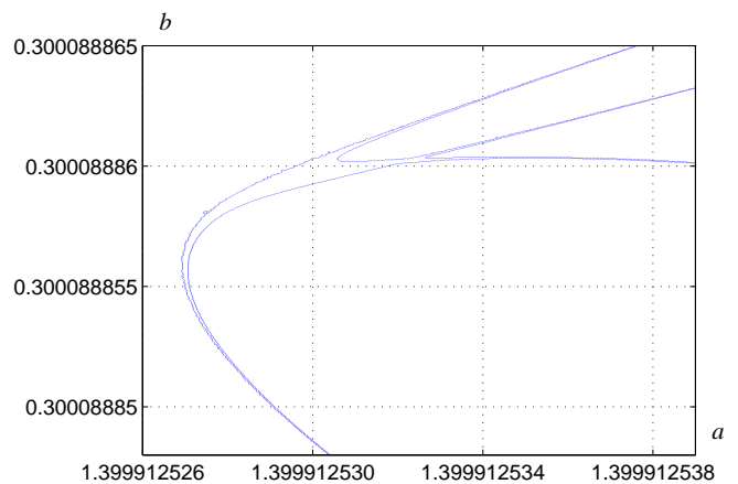
FIG. 15. Border of the period-39 complex existence region
