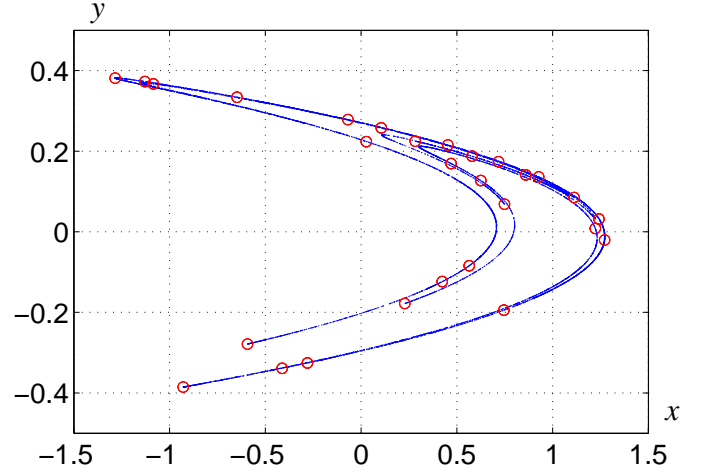
FIG. 10. Trajectory of the Hénon map with (a, b) = (1.4, 0.2999999774905) computed in the double-precision arithmetic for the initial condition (x_0, y_0) = (0, 0) , 10000 points after skipping 10^{10} iterations are plotted using blue dots, 10000 points after skipping 1.05 \cdot 10^{10} iterations are plotted using red circles, chaotic transient is observed for more than 10^{10} iterations; eventually, the trajectory converges to the period-28 sink
