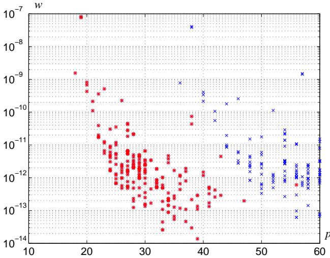
FIG. 6. Widths w of primary ( * ) and secondary ( \times ) existence regions versus period p
