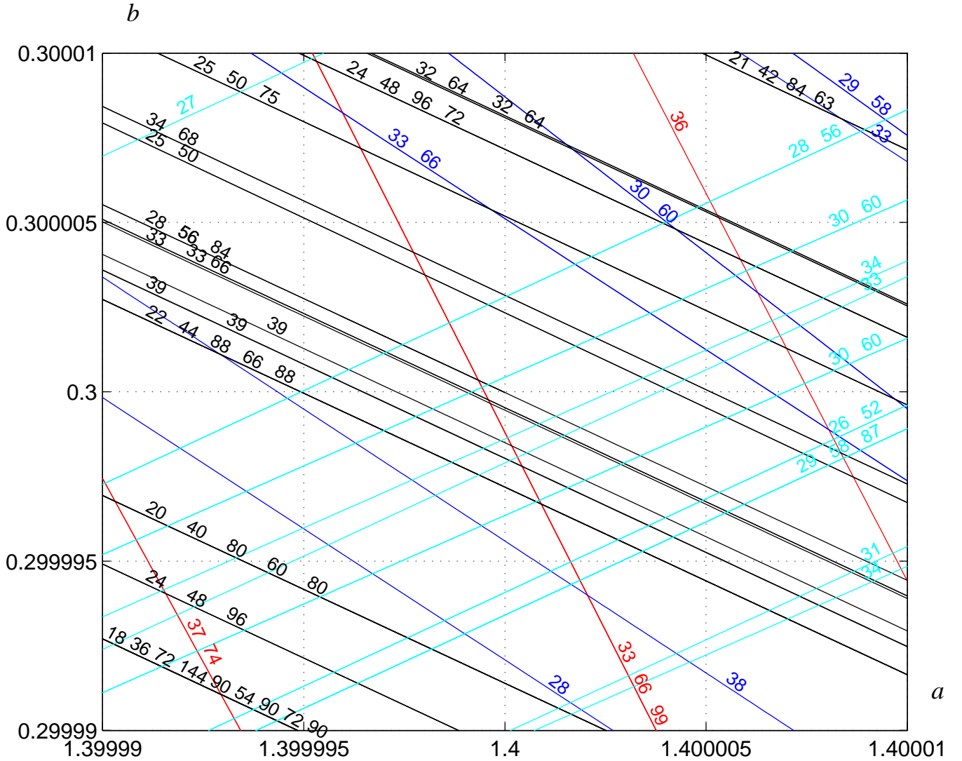
FIG. 4. Regions of existence of primary and secondary sinks in the rectangle (a, b) \in [1.39999, 1.40001] \times [0.29999, 0.30001]
