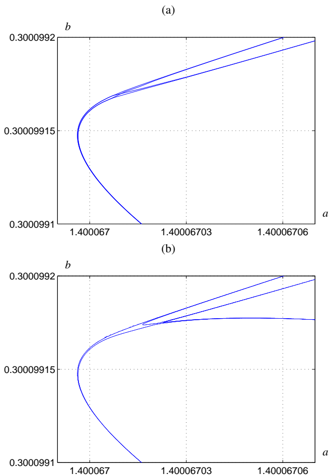
FIG. 14. Border of the period-35 complex existence region found using (a) the continuation method designed for narrow stripes and (b) grid continuation method
