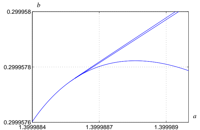
FIG. 16. Period-41 complex existence region
