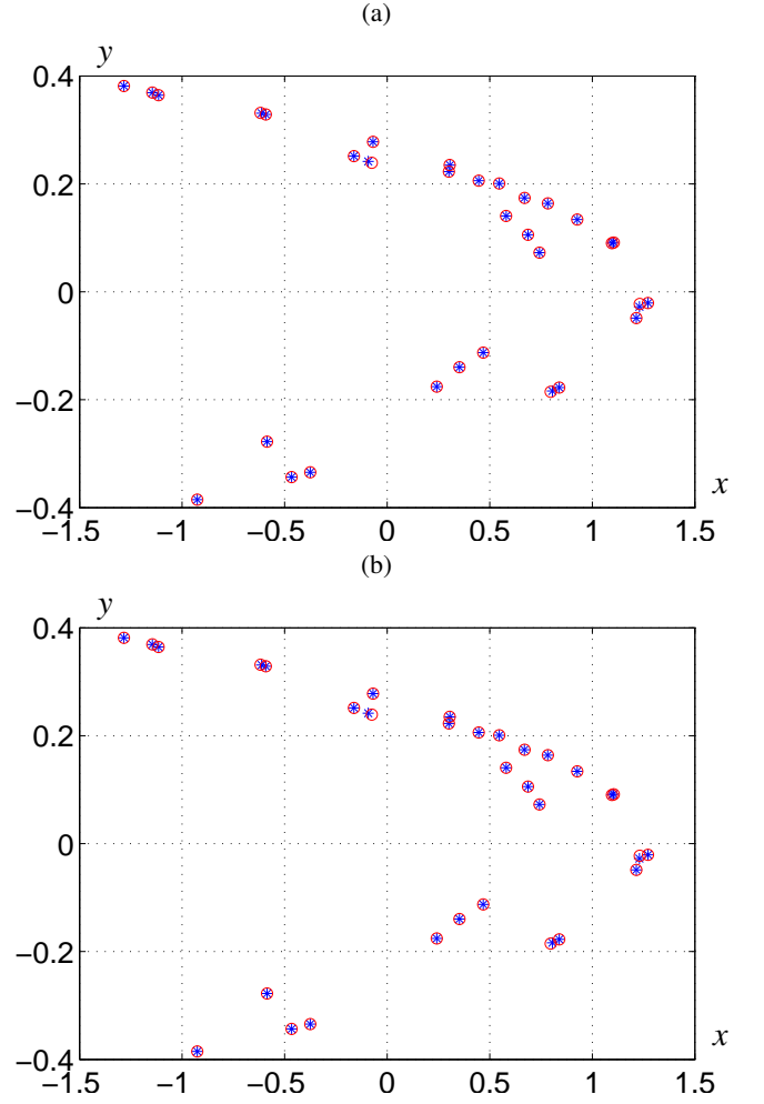
FIG. 13. (a) Period-32 sinks for (a, b) = (1.4, 0.3000081508615) (○) and (a, b) = (1.4, 0.300008095952) (*), (b) stable (○) and unstable (*) period-32 orbits for (a, b) = (1.4, 0.3000081508615) , the unstable sink was obtained using the continuation method from the stable sink for (a, b) = (1.4, 0.300008095952)
