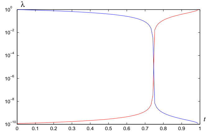
FIG. 8. Eigenvalues of the Jacobian matrix across the existence region of one of the period-19 sinks, t = 0 and t = 1 correspond to borders of the existence region
