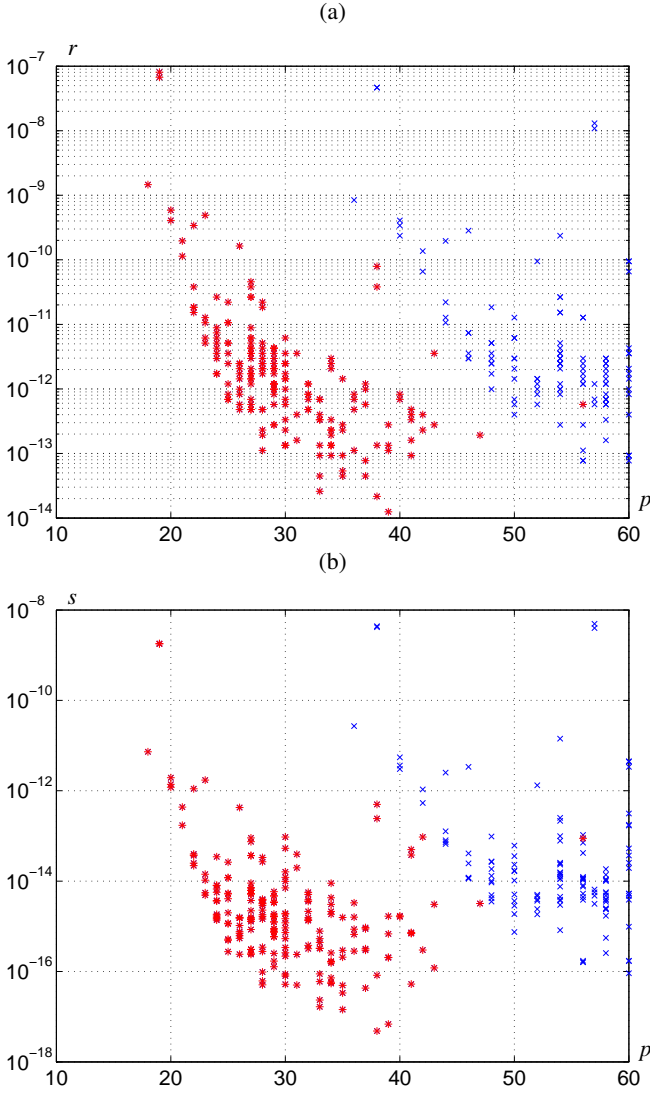
FIG. 9. The minimum immediate basin radius r_\varepsilon (a) and lower bound s_\varepsilon of the immediate basin area (b) versus period p for primary (*) and secondary (x) sinks
