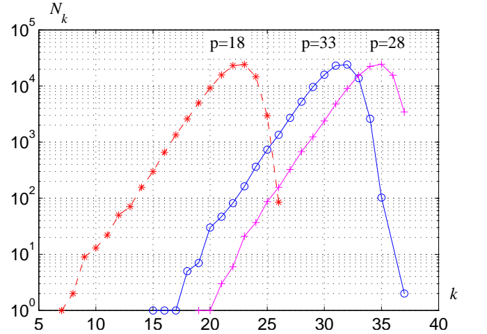
FIG. 11. The number N_k of random initial points with the convergence time in the interval [2^{k-1}, 2^k) ; (a, b) = (1.3999769102, 0.3) , period-18 sink (*); (a, b) = (1.3999994869436, 0.3) , period-33 sink, (o); (a, b) = (1.4, 0.2999999774905) period-28 sink, (+)
