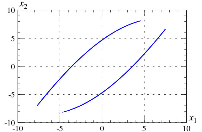
Fig. 2. A 1000000 points computer generated trajectory of P
