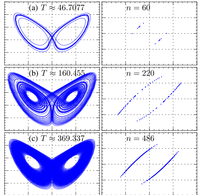
Fig. 5. Examples of long periodic orbits
